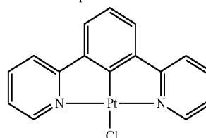
(1,3-Bis(2-pyridinyl)phenyl-C,N,N')(chloro)platinum
