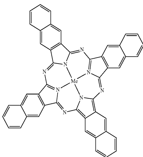
[Naphthalocyanine]
