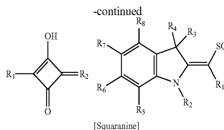
[Squaraine]
