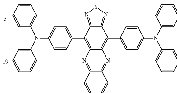
4,4'-((1,2,5)thiadiazolo[3,4-b]phenazine-4,11-diyl)bis(N,N-diphenylaniline)
